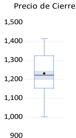
Diagram 1 Box and whisker plot chart boxplot of ECUINDEX stock index
